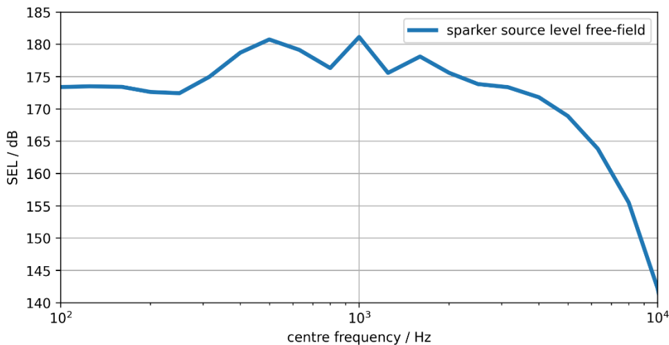
Figure 3.3 Source spectrum @ 1 m Dura-Spark 400+400, 2000 J
