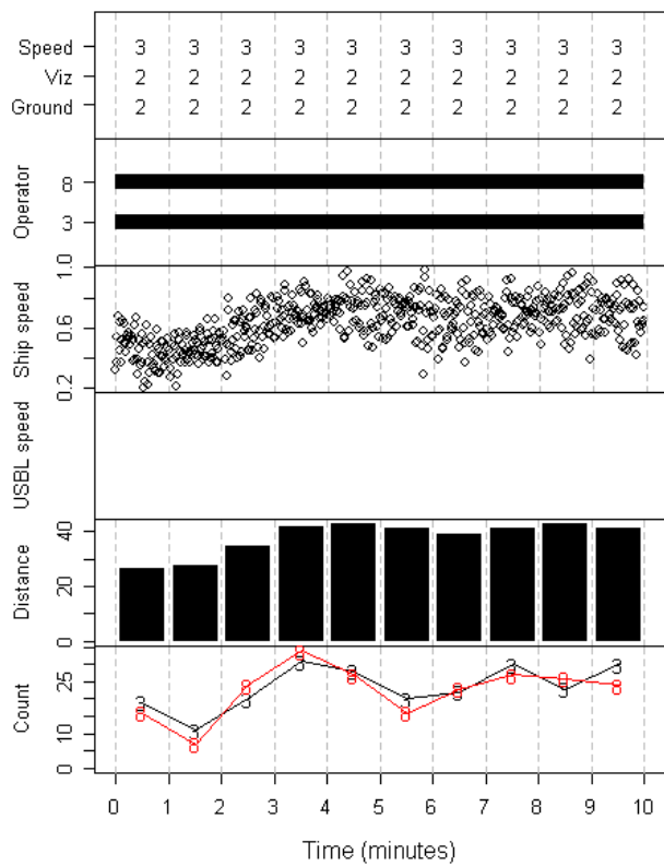
Figure 1.R tool quality control plot of station 150 UWTV Survey of the Smalls Grounds FU20-22 2008
