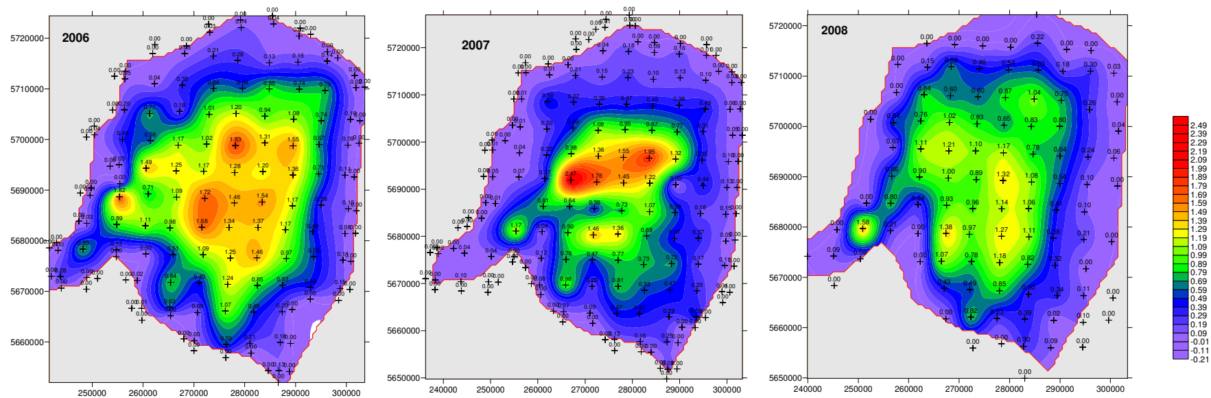
Figure 8: Contour plots of the kriged density estimates for the Smalls Grounds from 2006-2008.
