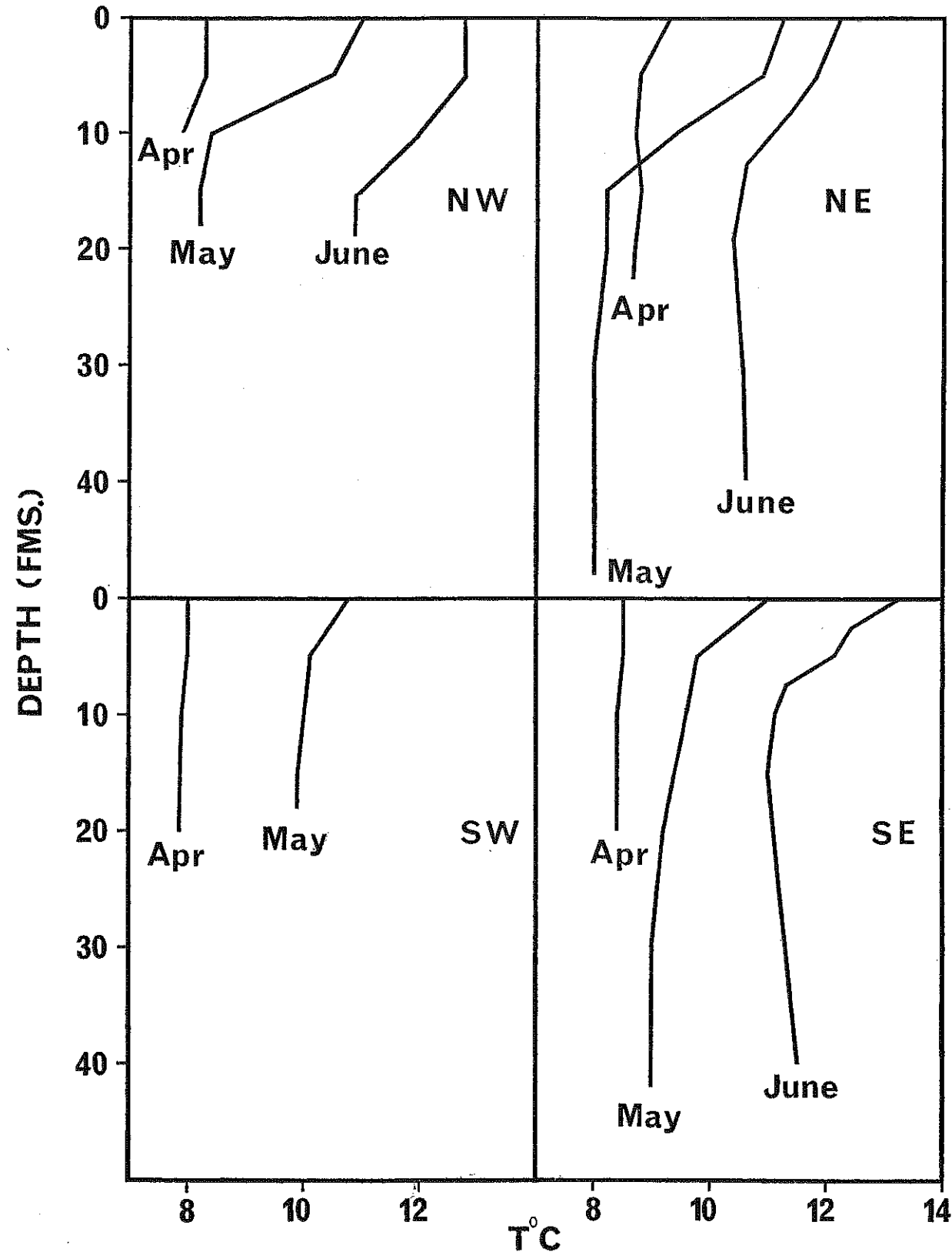
Fig. 10. Temperature (°C) by depth in four quarters of area, April-June 1971.
